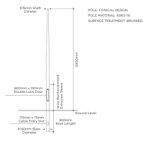
COLUMN DIMENSIONS
