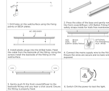
LED Linear Batten Fitting
