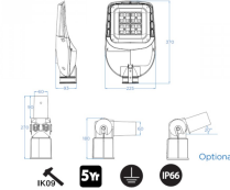
LED Eco Street Lantern Light DIMENSIONS
