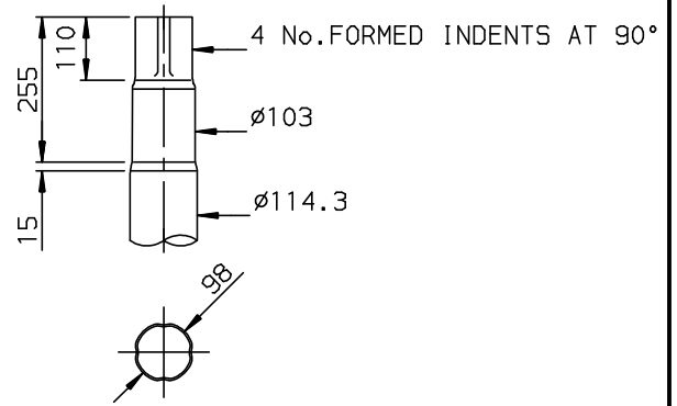
DETAIL OF TOP OF COLUMN. SCALE 1:10
